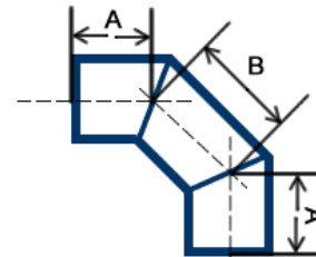
Elbow - 3 Three-piece 46° to 90°
