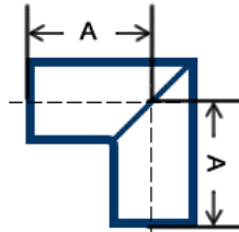
Elbow - 2 Two-piece 46° to 90°
